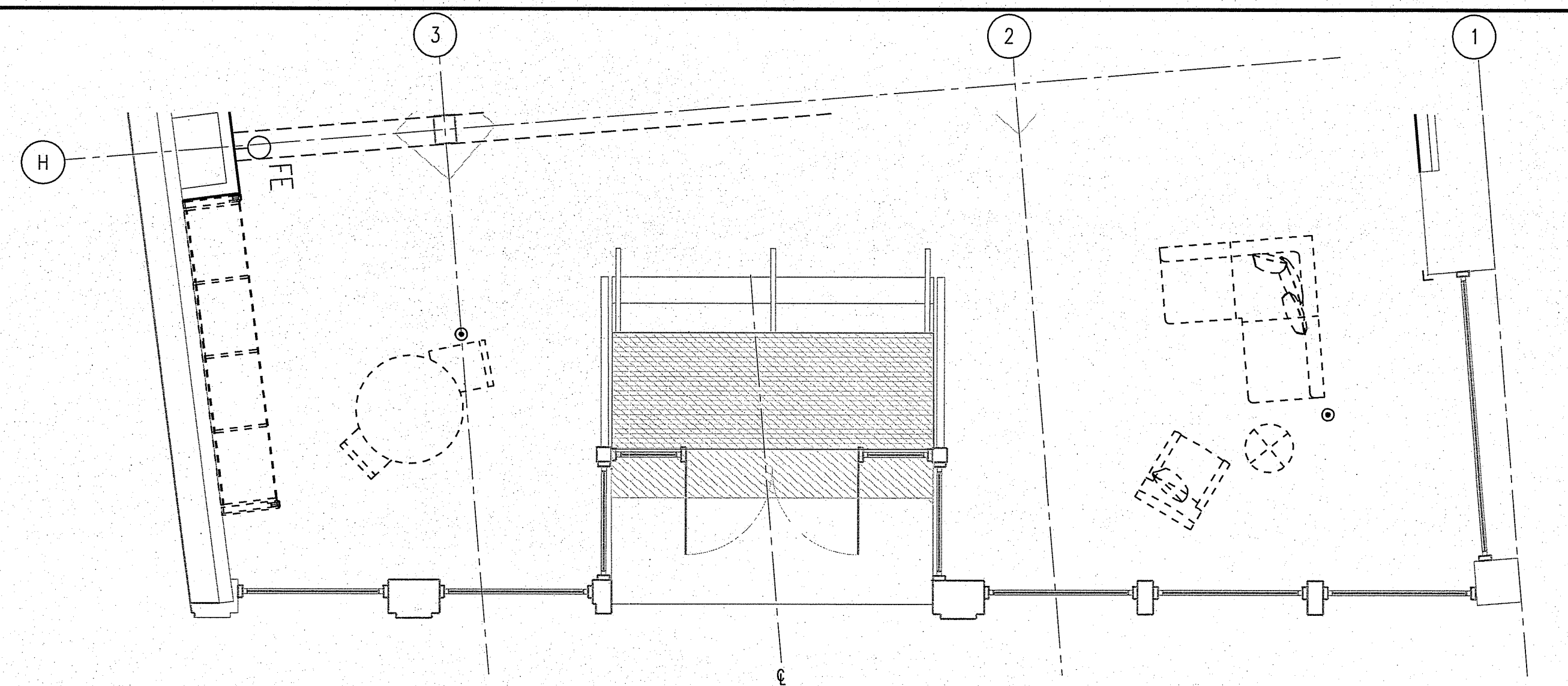
D1 PARTIAL STOREFRONT PLAN - ENTRY NO 1 1/4"=1'-0" 0 2' 4' 8'
